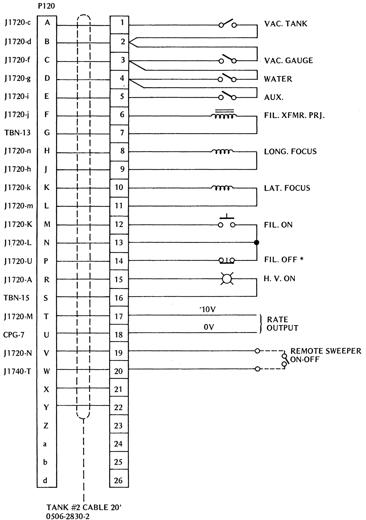
Figure 2-5. CV-14 A and B interlock terminal strip connection diagram
