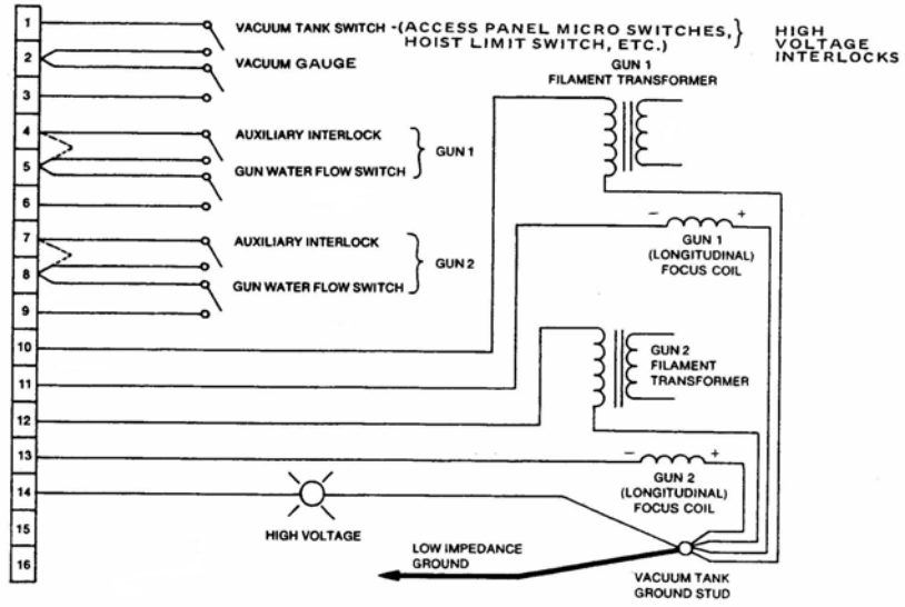
Figure 2-4. Interlock terminal strip connection diagram
