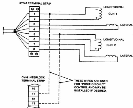
Figure 2-5. XYS-8 terminal strip connection diagram
