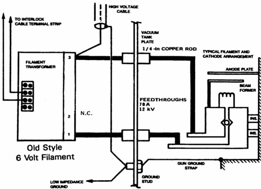
Filament transformer connection diagram, 420 VA
