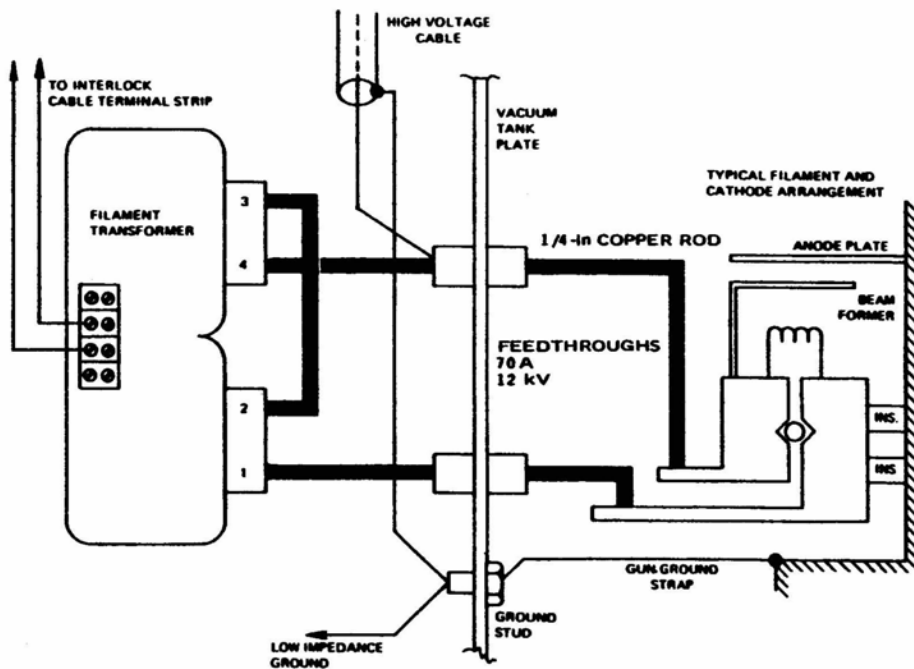
Figure 2-2. Filament transformer connection diagram, 840 VA
